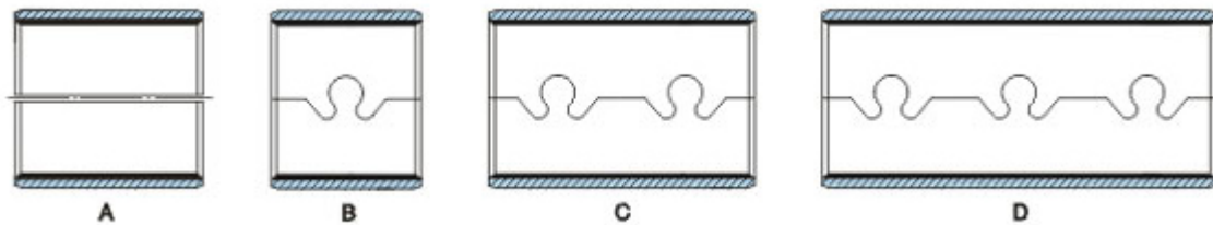
SF-3 卷制轴承搭口形式 Joint forms of SF-3 wrapped Bearings
