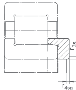
Winkelring
