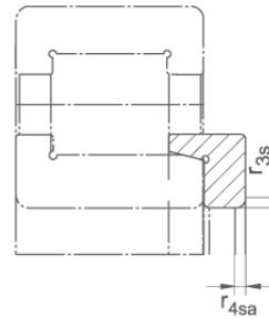
Angular ring
