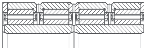
Walzwerkslager/Rolling mill bearing
