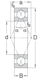
Reihe/Series Q10, Q2, Q3 Druckwinkel/Contact angle = 23°
