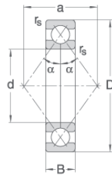
Reihe/Series QJ10, QJ2, QJ3 Druckwinkel/Contact angle = 35°
