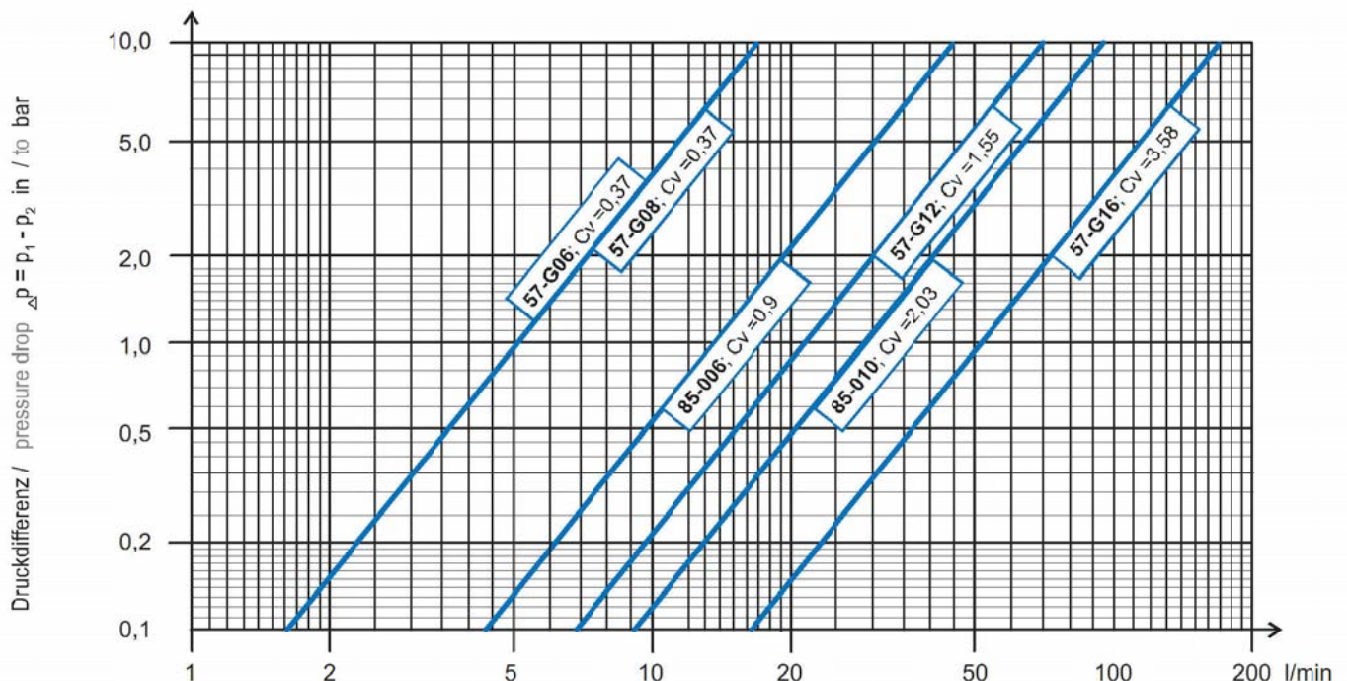
效能圖表 / Performance diagram
